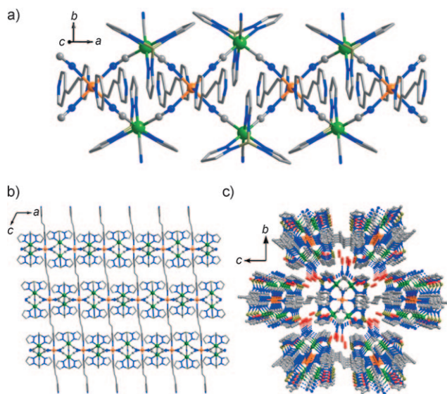
Figure 1. a) Side view of the double zigzag chain in 1 ·5H 2 O along the c axis. b) Side view of the layer structure in 1 ·5H 2 O along the b axis. c) Packing structure of 1 ·5H 2 O along the a axis. The dashed lines represent hydrogen bonds between uncoordinated water molecules and terminal cyanide nitrogen atoms. Fe green, Co orange, N blue, O red, C gray, and B dark yellow.
